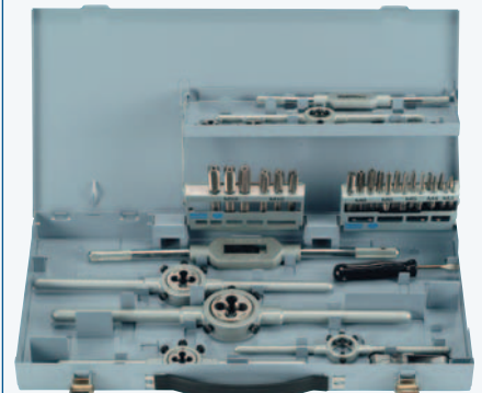
HSS-G DIN Gewindebohrersatz, 37-tlg. HSS-G DIN Taps and dies set, 37 pcs. Assortimenti maschi HSS-G, 37 pz. Stahlblechkassette | Metal cassette | Cassetta metallo Art.-Nr. 00 708000311 00 € 171,33
